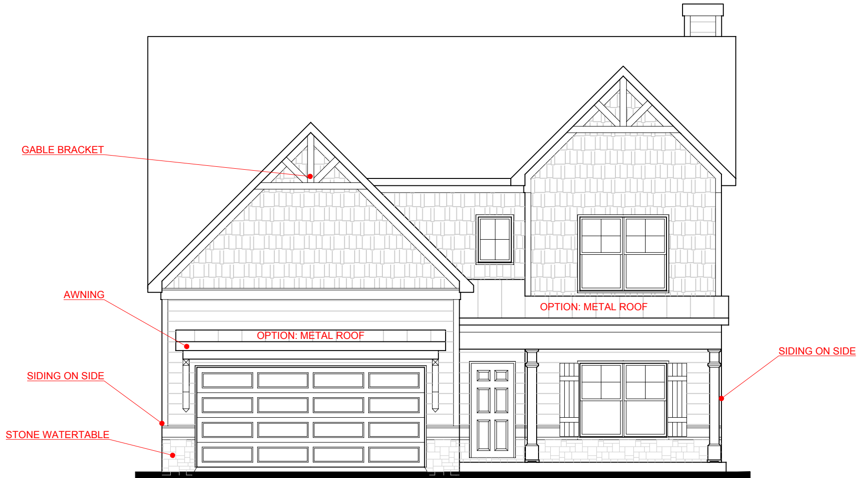
FRONT ELEVATION- B VERSION
