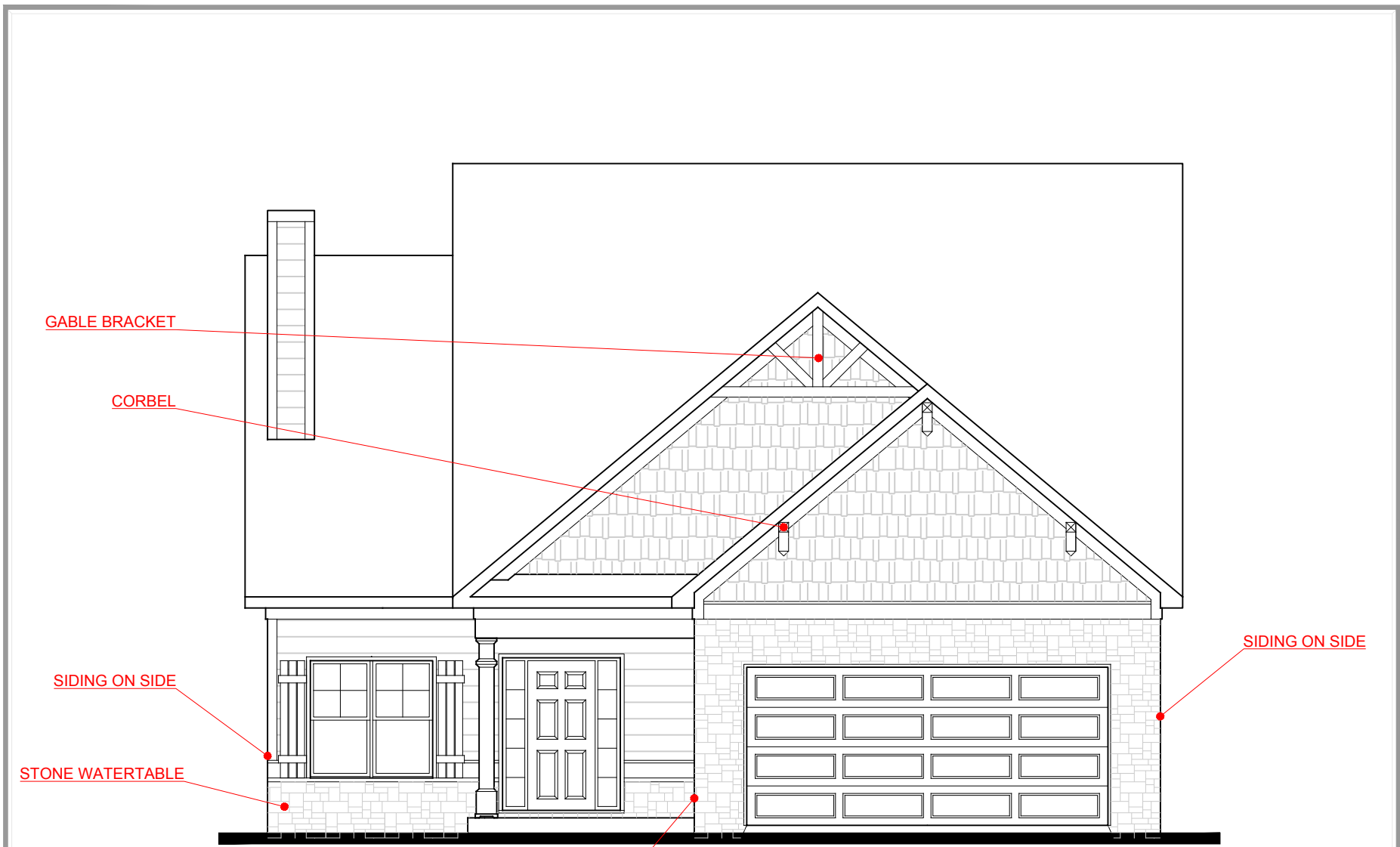
FRONT ELEVATION- B VERSION
