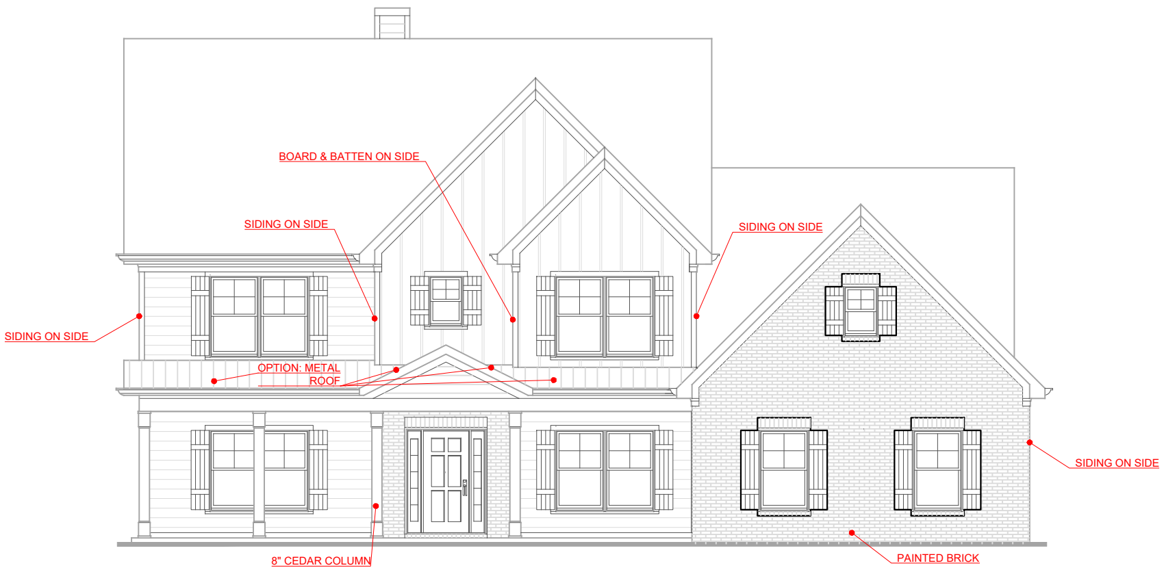
FRONT ELEVATION- F VERSION
