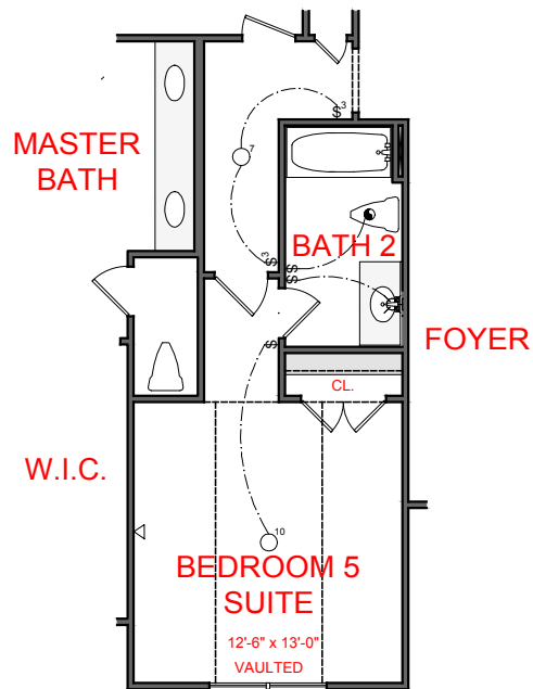
OPTION: BEDROOM 5 SUITE
