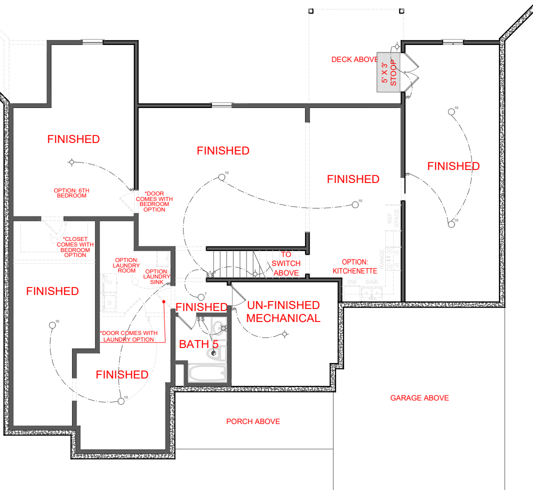
OPTION THREE: FINISHED BASEMENT PLAN 2,118 SQ. FT. FINISHED
