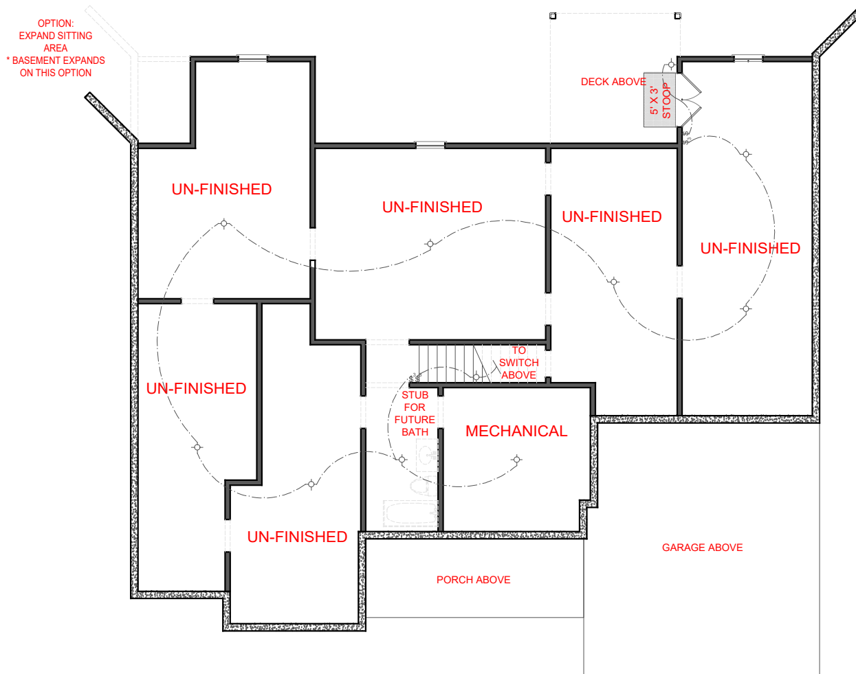
OPTION ONE: UN-FINISHED BASEMENT PLAN
