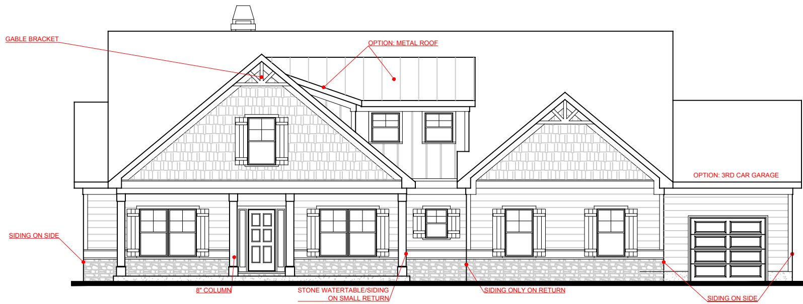
FRONT ELEVATION- B VERSION
