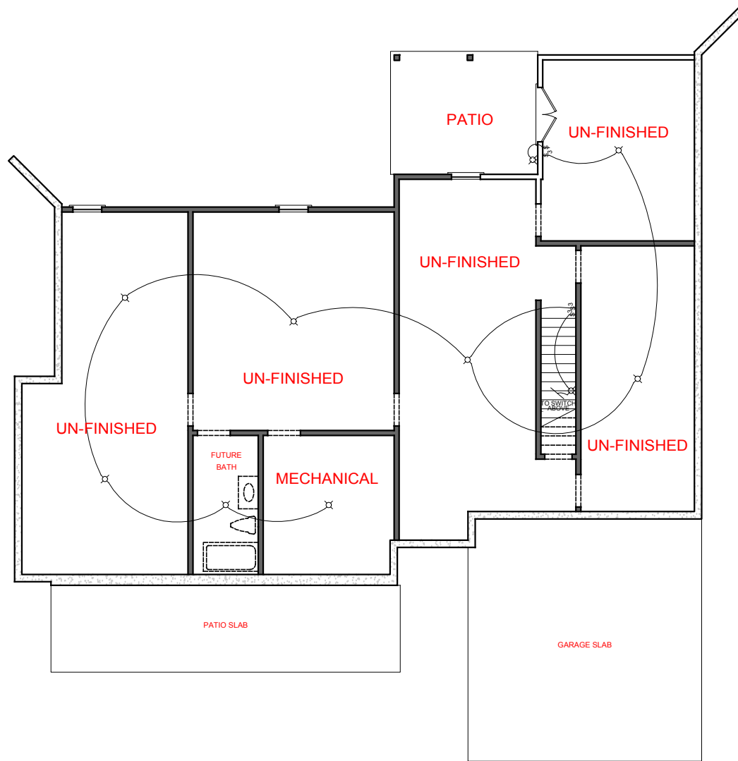
UN-FINISHED BASEMENT PLAN
