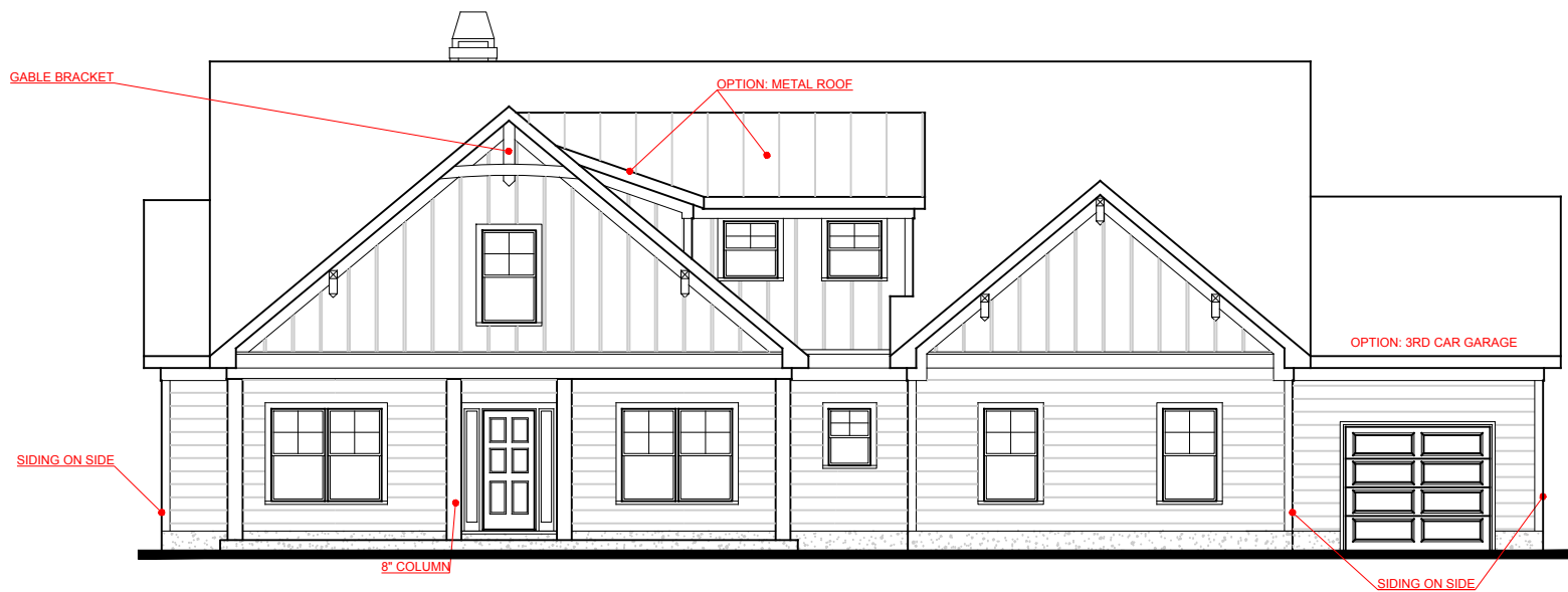
FRONT ELEVATION- A VERSION
